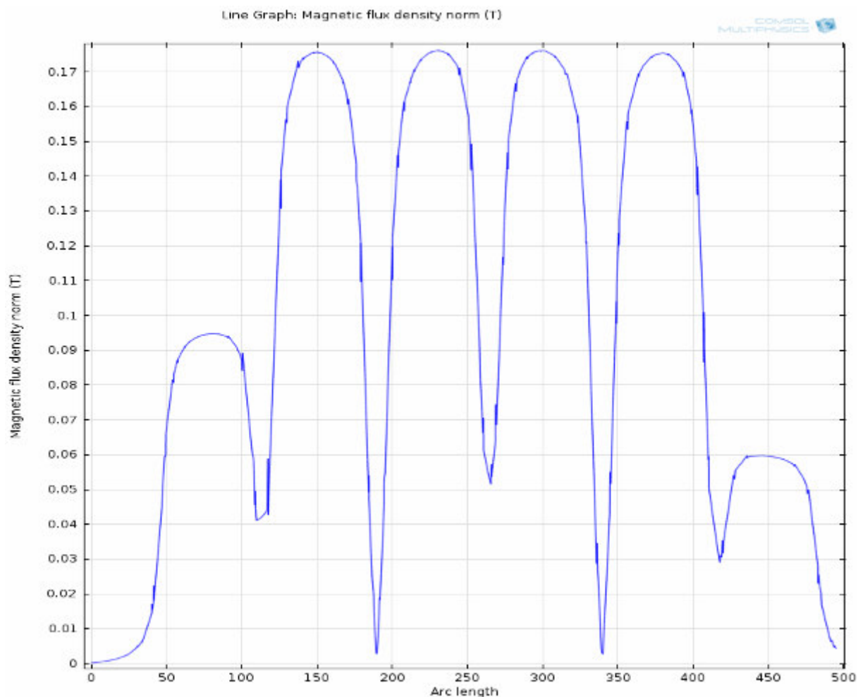
Picture 4 – The graph of magnetic induction distribution on the length of MAD
