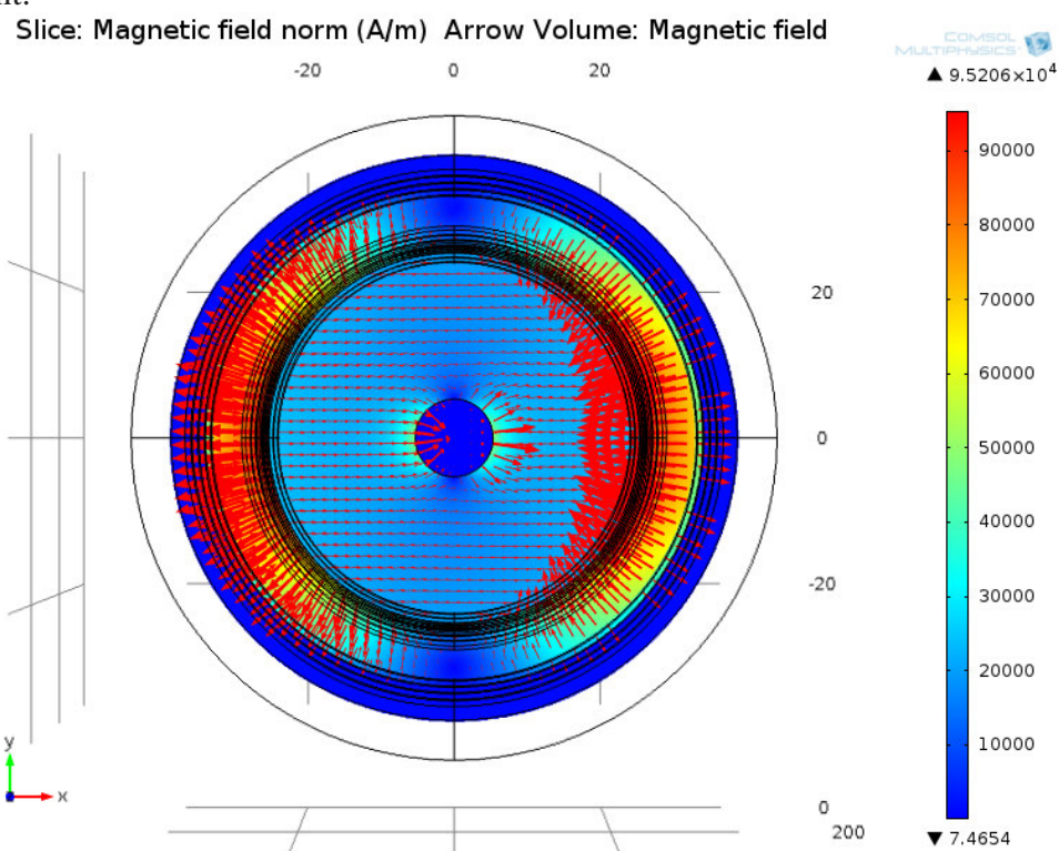
Picture 8 – Influence of magnetic field on mechanical impurities
