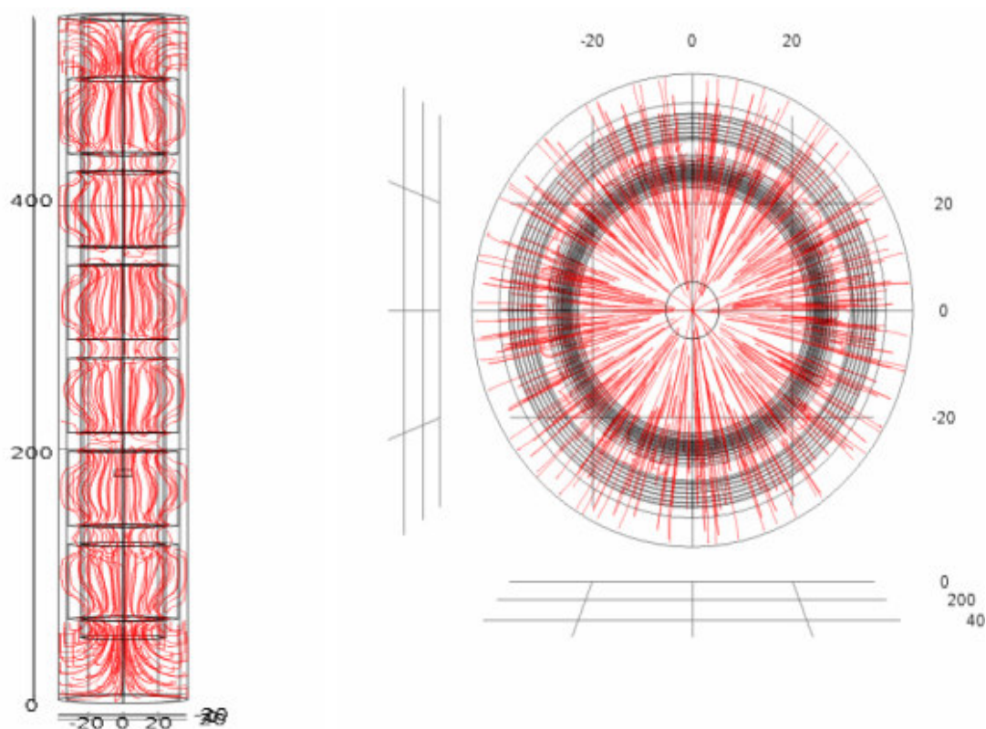
Picture 9 – Lines of the magnetic field
