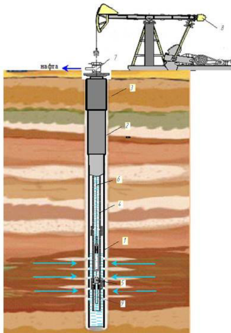
Picture 2 – MAD operational procedure in the well:
