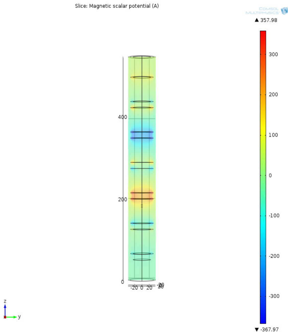
Picture 7 – Distribution of the scalar potential in the MAP
