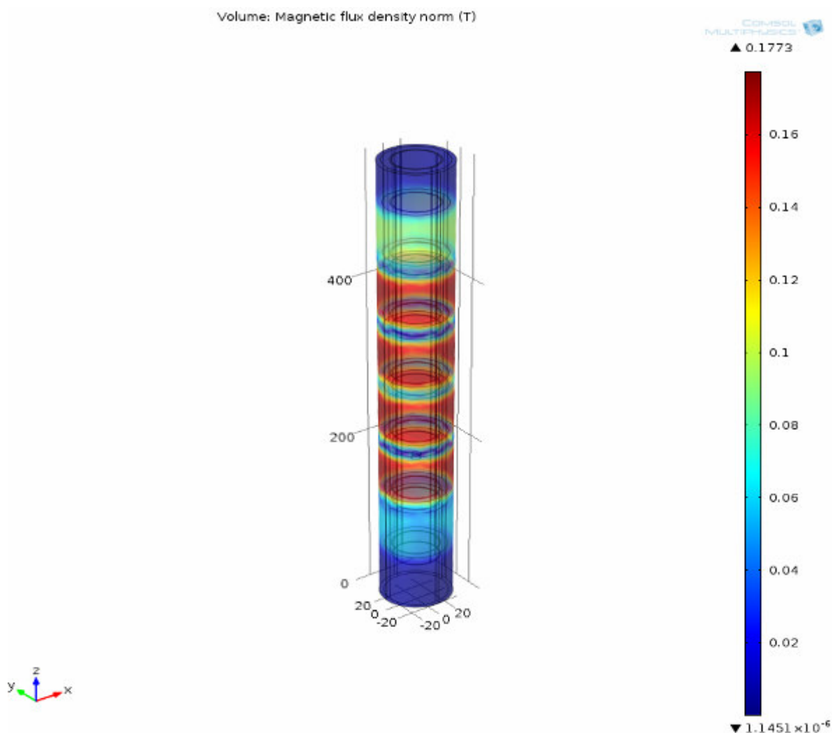
Picture 10 – 3D model of magnetic induction distribution
