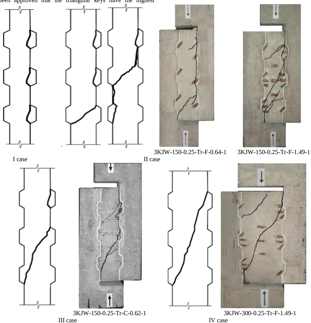
Fig. 3: The failure character of the three-keyed joints made from fibre concrete with the trapezoidal keys.
