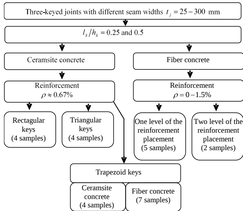
Fig. 2: The experiments program for samples of 6 th series.
