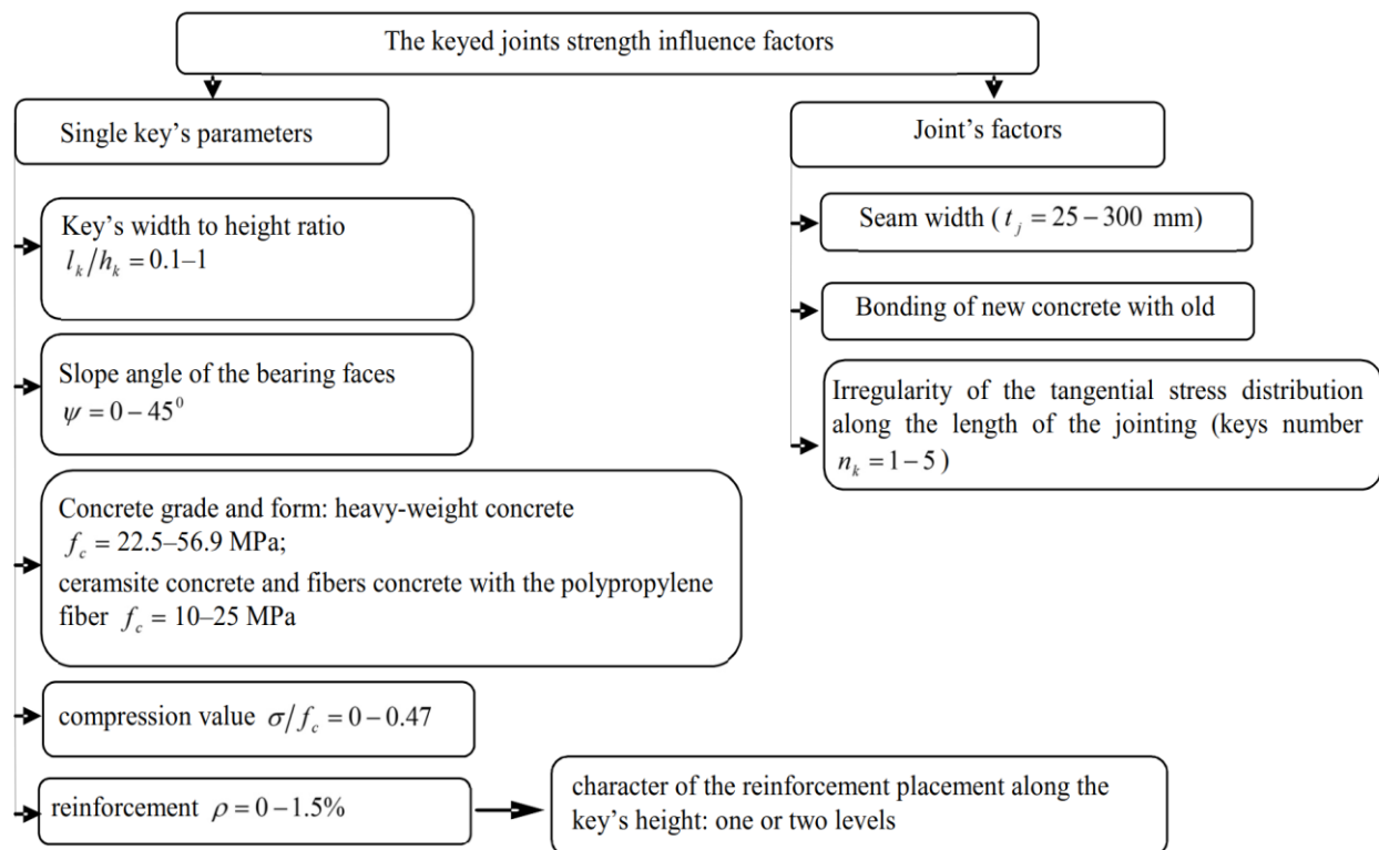
Fig.1: The strength influence factors of the concrete and reinforced concrete keyed joints.
