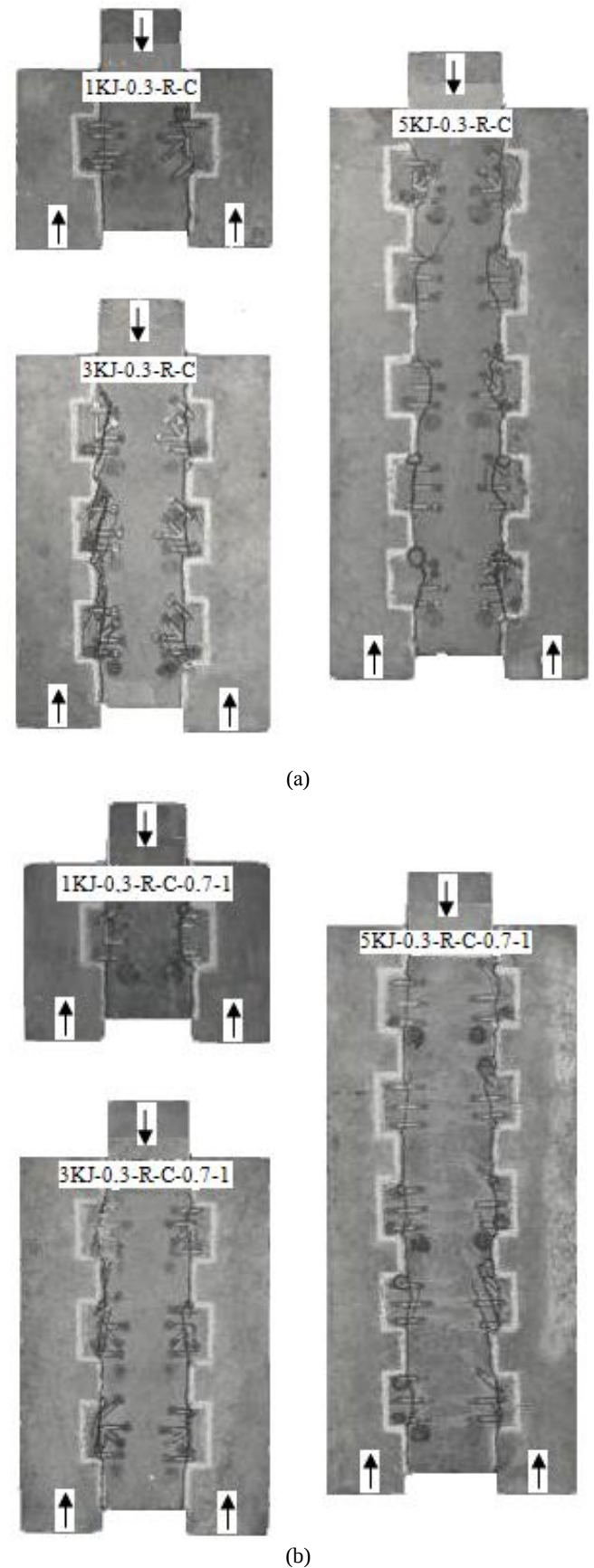
Fig. 6: The failure character of the samples with different number of keys: (a) concrete keyed joints samples; (b) reinforced concrete keyed joints samples.
