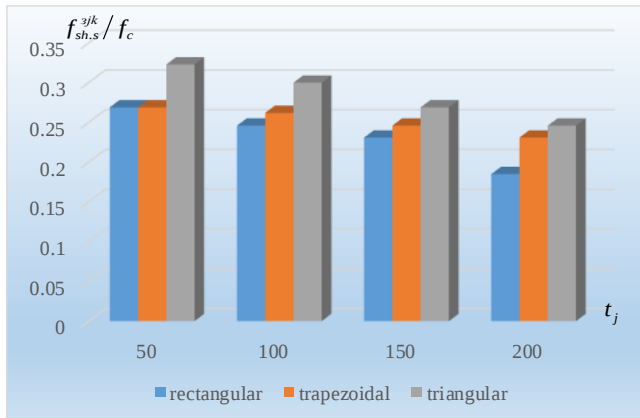
Fig. 4 The strength of three-keyed joints of ceramsite concrete f_{sh,s}^{ijk} on the width of the seam t_j .
