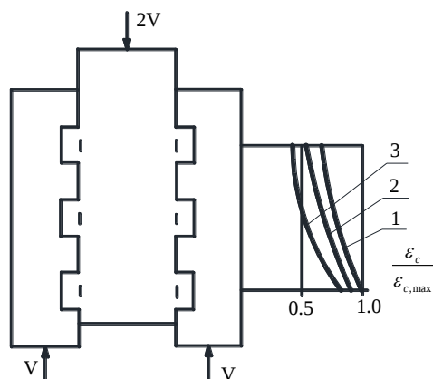
Fig. 7: Concrete strain distribution along the joint length in the sample 3KJ-0.3-R-C-0.7-1: 1 – V/V_u = 1 ; 2 – V/V_u = 0.87 ; 3 – V/V_u = 0.79 .
