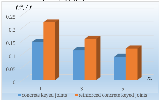
Fig.5: Keyed joints strength f_{sh,s}^{nk} depending on the number of keys.
