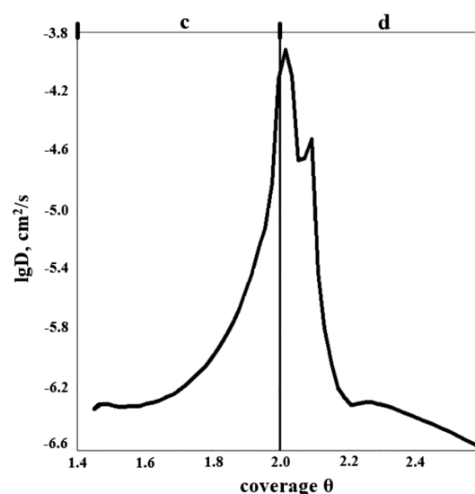
Fig. 4. Dependence of the diffusion coefficients on \theta_{\text{Cu}} at the boundary of the second and third geometric monolayers at T = 857 K
