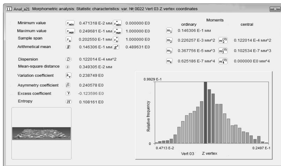
Fig. 5. Statistical characteristics and histograms of proportional coordinates frequencies for peaks Z of the triangulation model of the working surface of the initial wheel (a); and the wheel after grinding (b)
